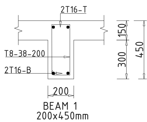
BEAM LAYOUT DETAILS FOR FIRST, SECOND AND THIRD FLOORS
