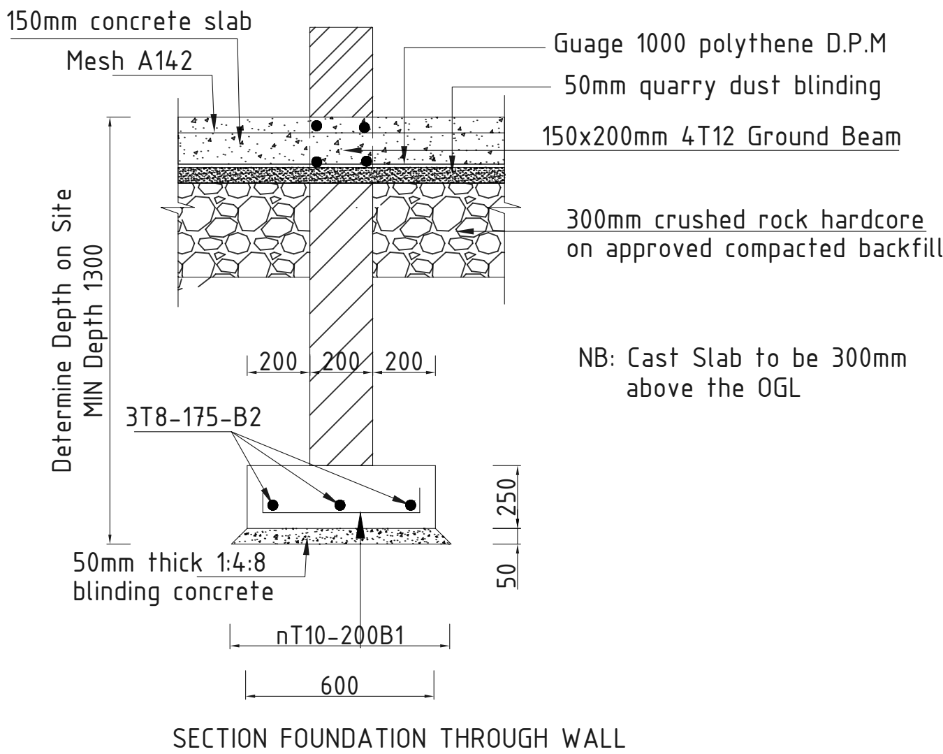
SECTION FOUNDATION THROUGH WALL
