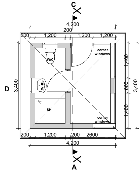
FLOOR PLAN
