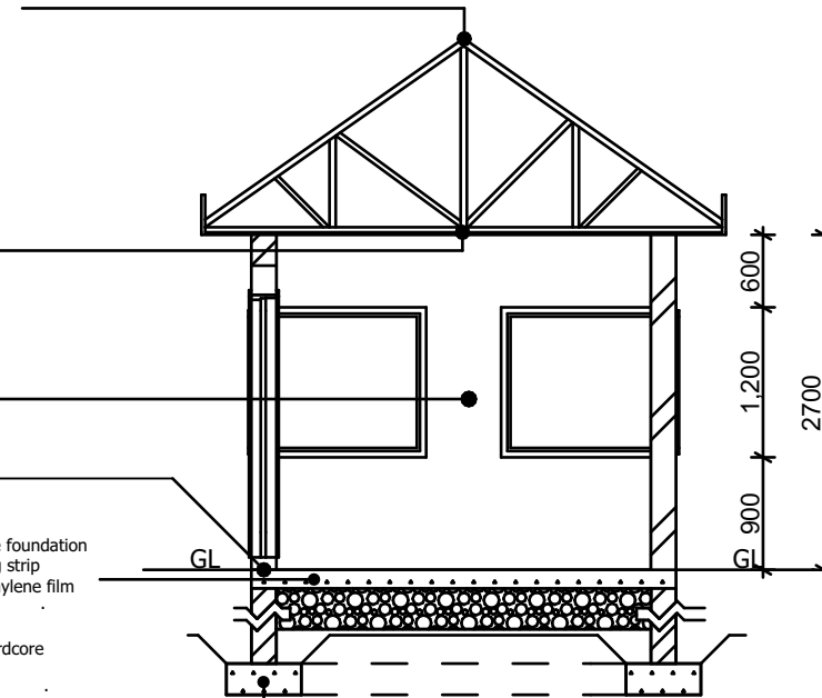
SECTION X-X
