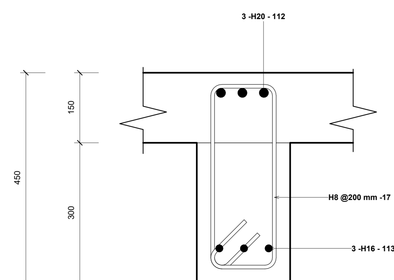
4 BEAM 4 SPAN DETAILS 1 : 5
