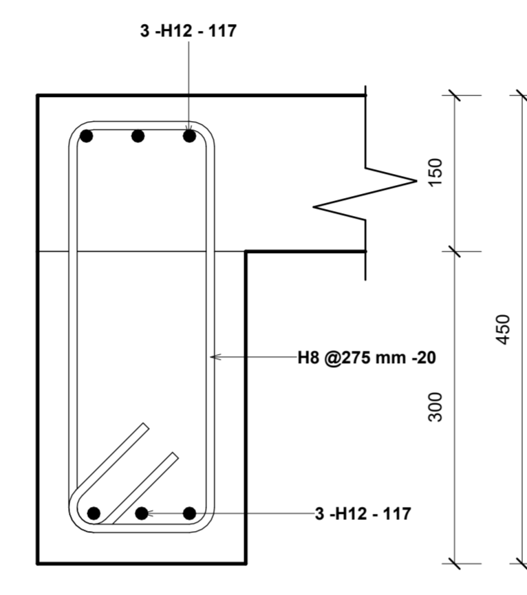
4 BEAM 1 AT SPAN 1 : 5
