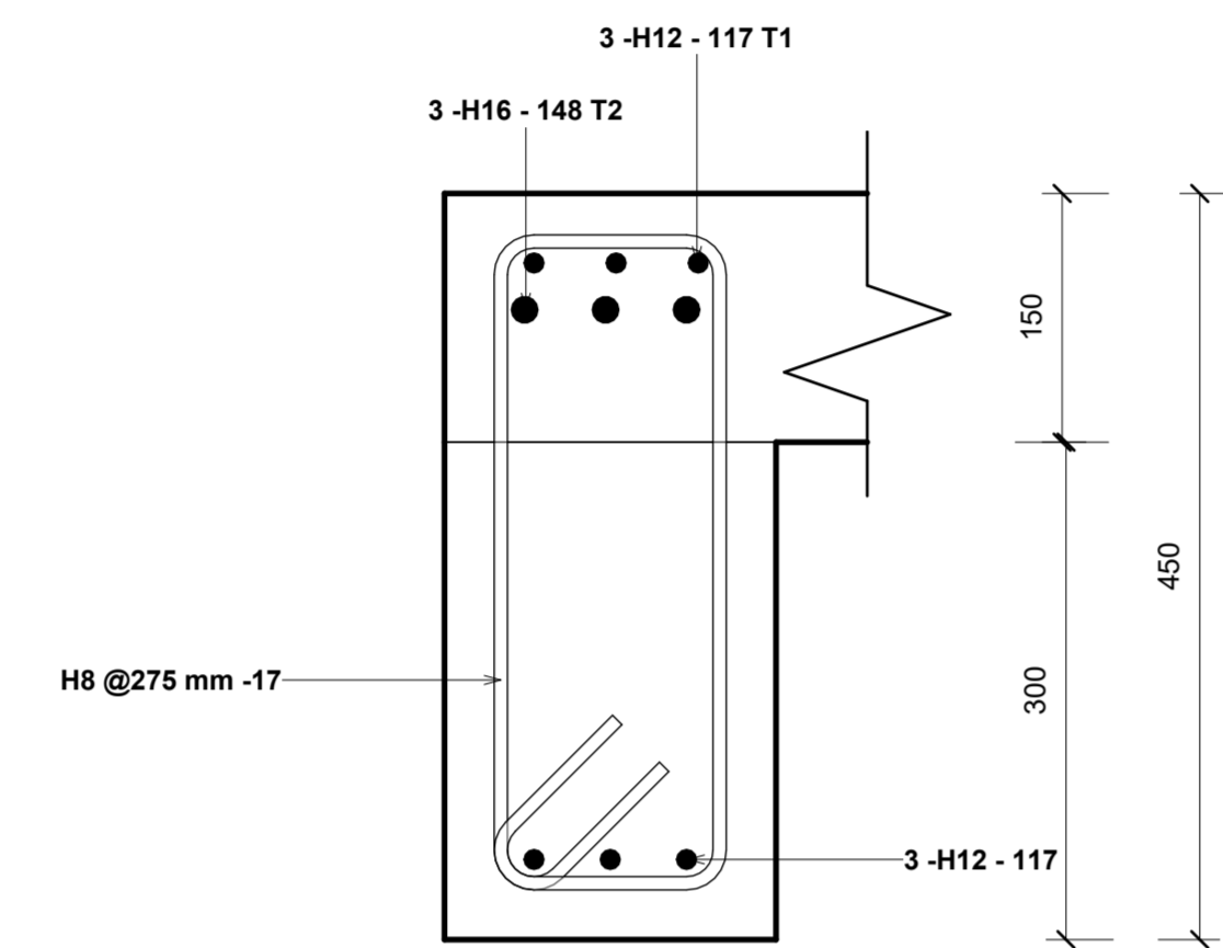
3 BEAM 1 SUPPORTS 1 : 5
