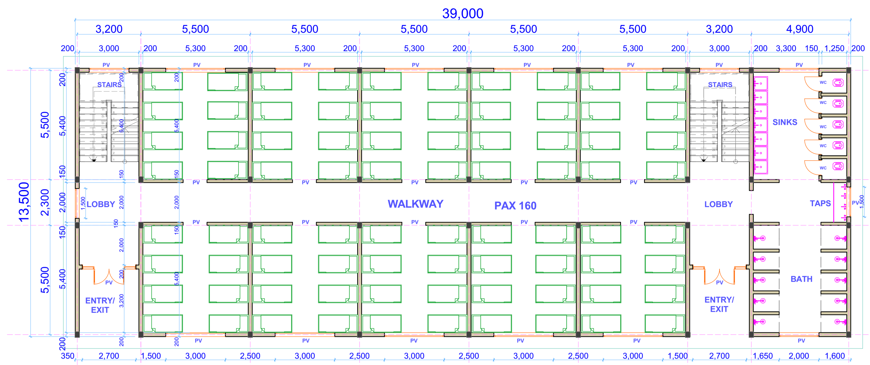
GROUND FLOOR LAYOUT
