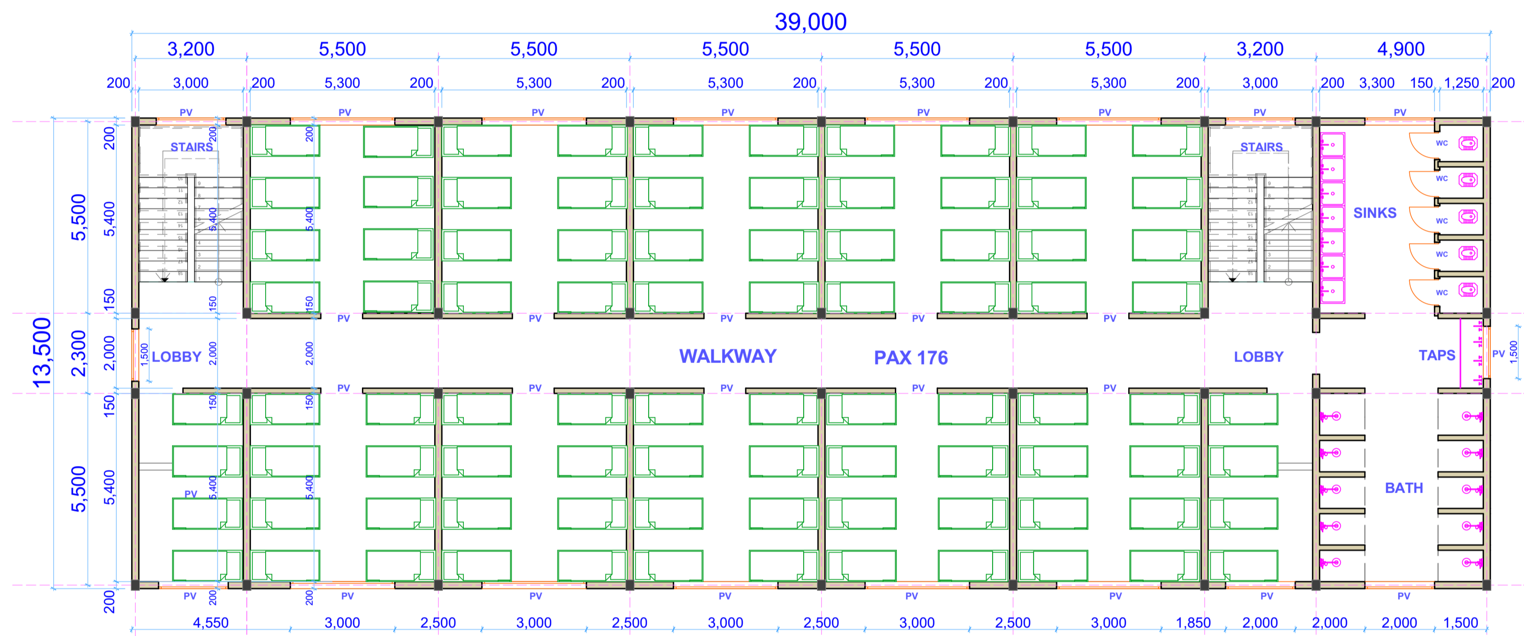
1ST-4TH FLOOR LAYOUT
