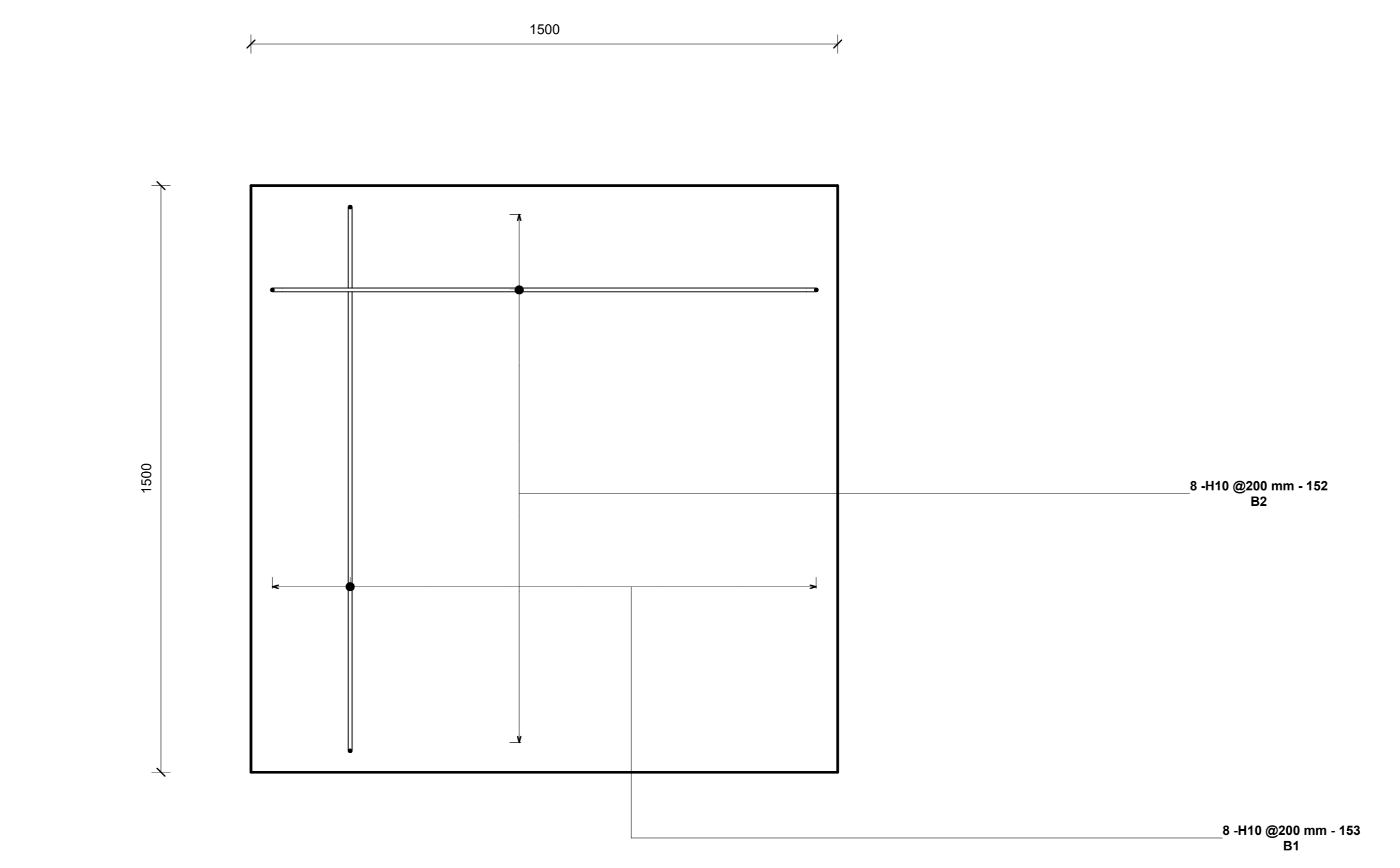
3 PAD P1 FOOTING DETAILS 1 : 10
