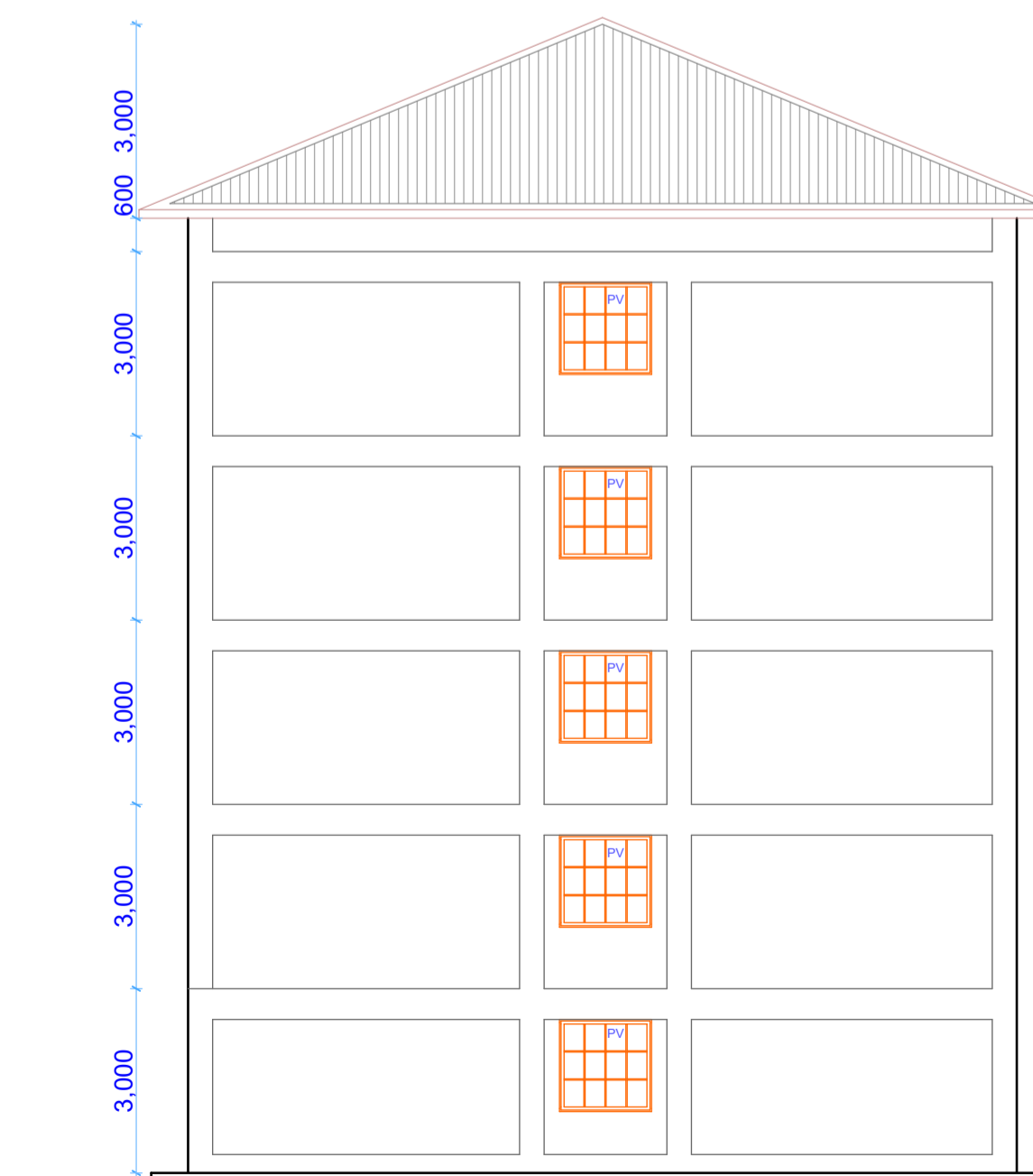
SIDE A ELEVATION
