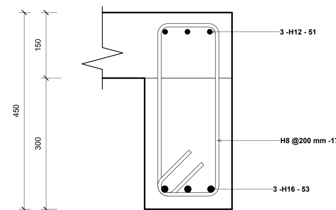
2 BEAM 3 MIDSPAN DETAILS 1 : 5
