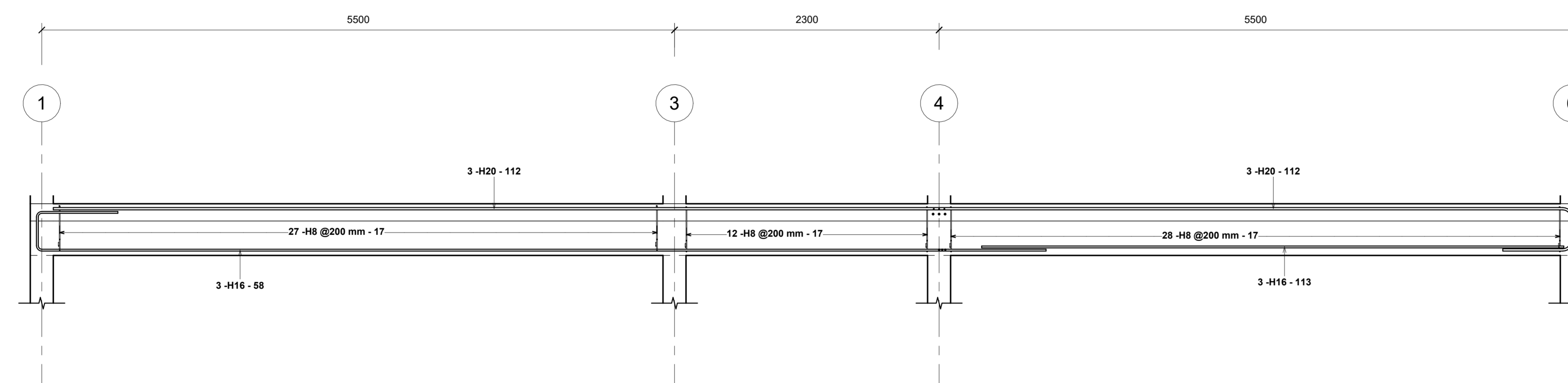
3 BEAM 4 DETAILS 1 : 25
