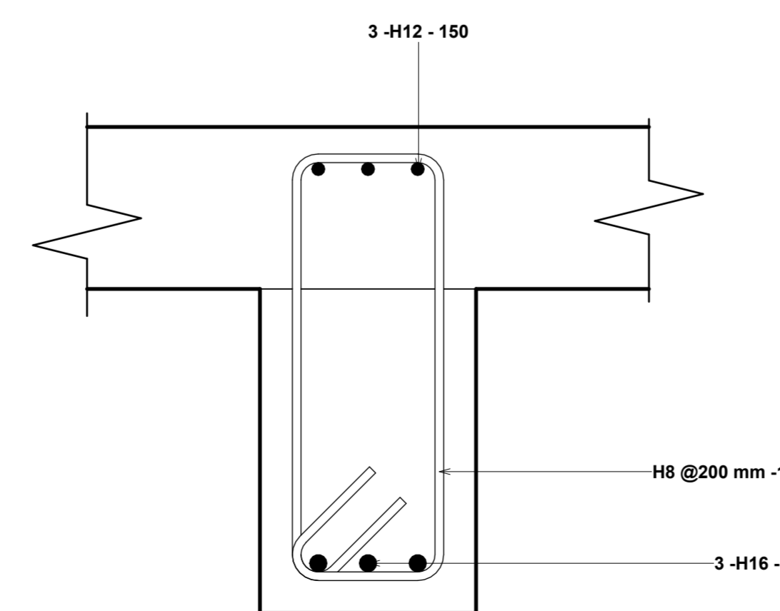
6 BEAM 2 MIDSPAN DETAILS 1 : 5
