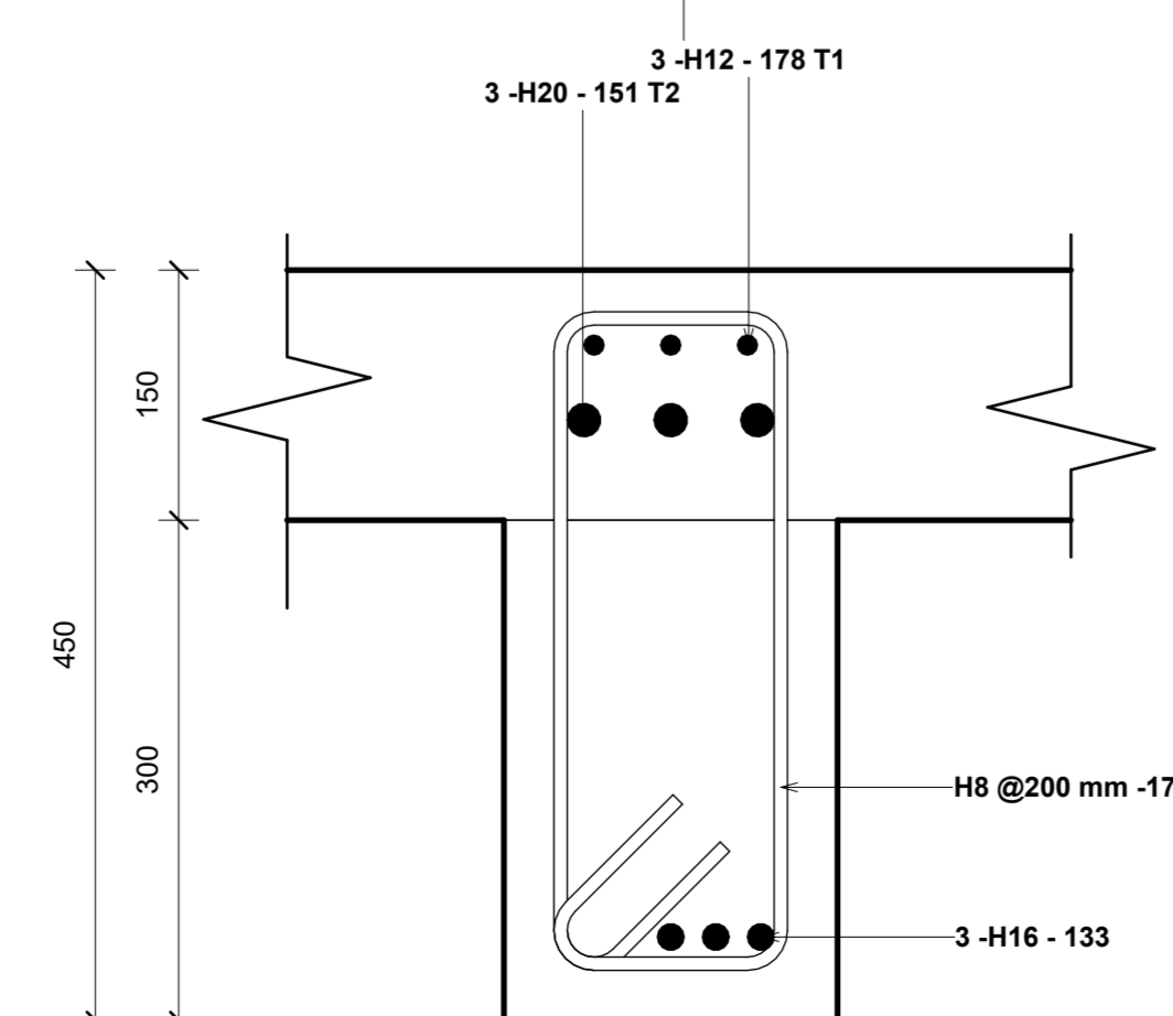
5 BEAM 2 SUPPORT DETAILS 1 : 5
