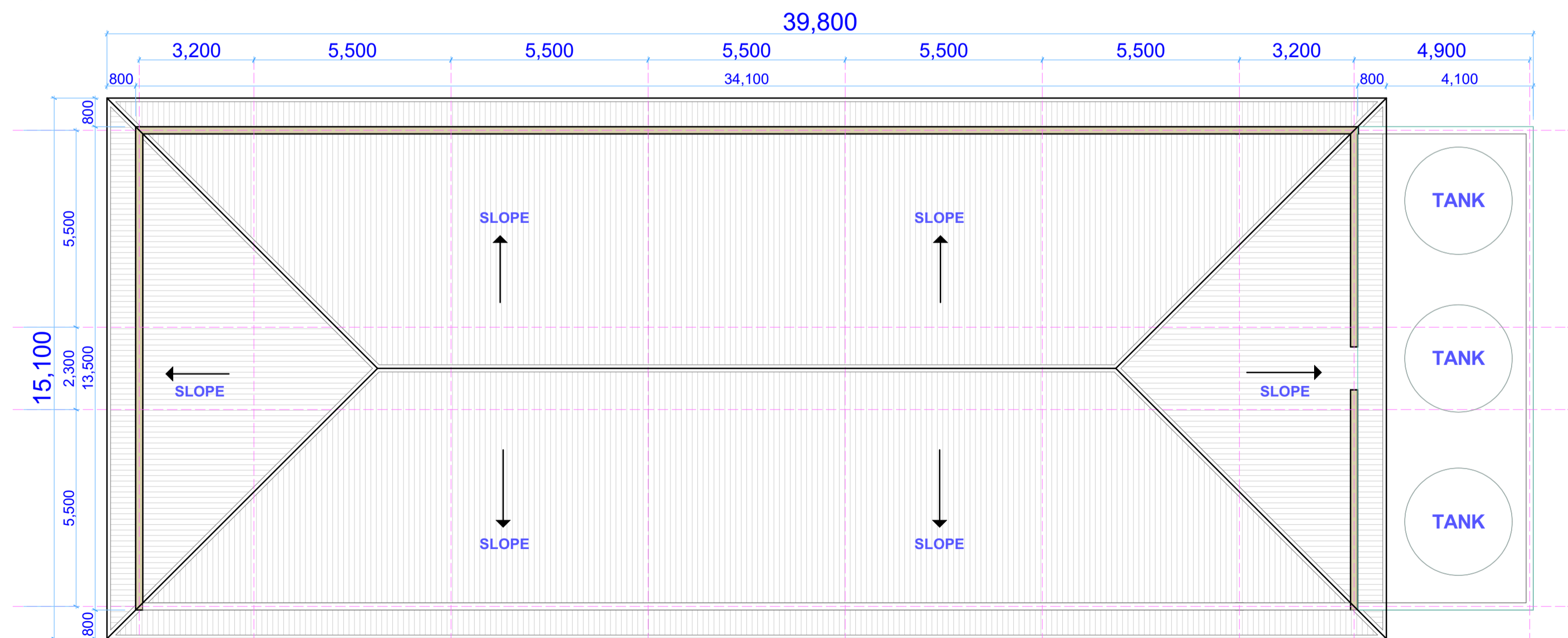
ROOF LAYOUT
